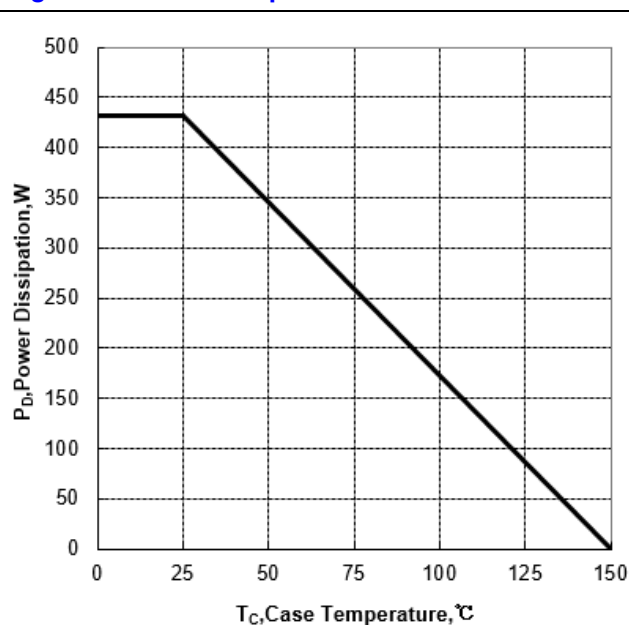
Figure 2 Power Dissipation
