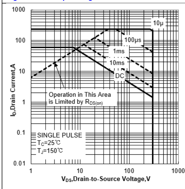
Figure 1 Safe Operating Area
